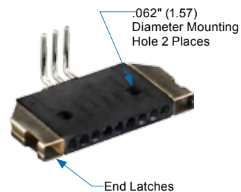
Figure 3 Right Angle PCB Header with End Latches and Mounting Holes. Part Number 171-004-11P-.250-BLMH.
