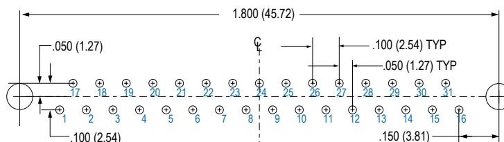
31 SOCKET M83513/25-E
