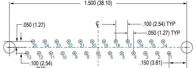
25 PIN M83513/22-D
