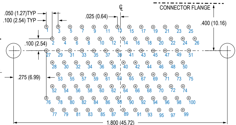
100 PIN M83513/12-H
