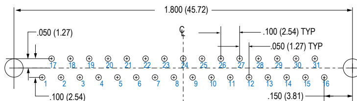
31 SOCKET M83513/25-E
