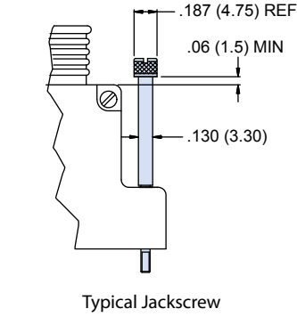
Typical Jackscrew
