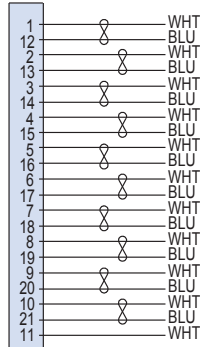
21 Contacts
