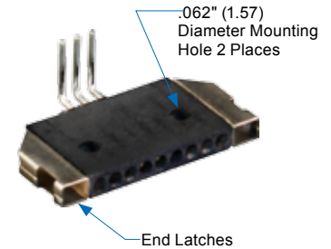
Figure 3 Right Angle PCB Header with End Latches and Mounting Holes. Part Number 171-004-11P-.250-BLMH.
