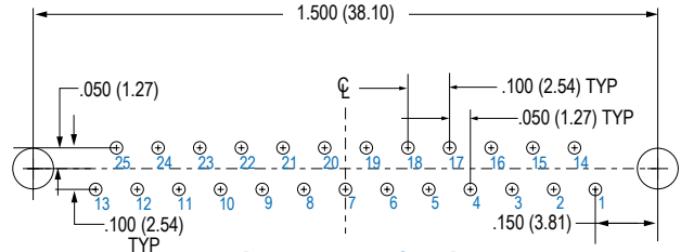
25 PIN M83513/22-D
