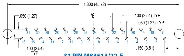
31 PIN M83513/22-E
