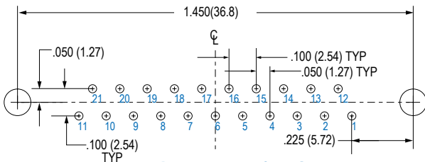
21 PIN M83513/22-C
