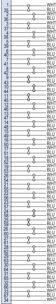
67 Contacts
