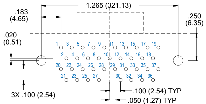
37 PIN
