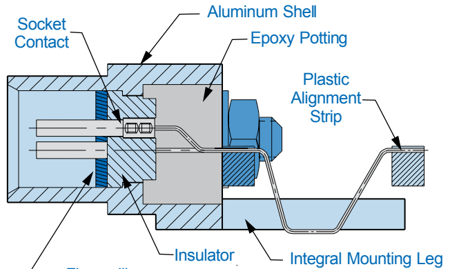
Socket Connector
