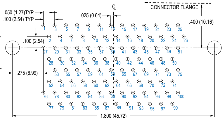
100 PIN M83513/12-H
