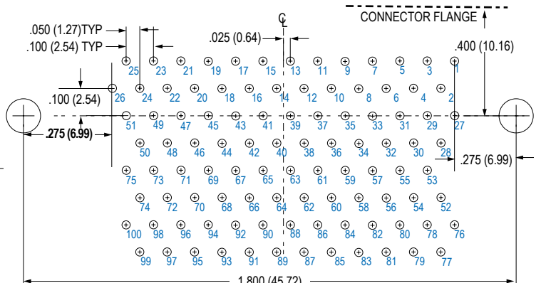
100 SOCKET M83513/15-H
