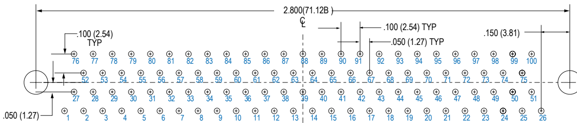
100 SOCKET M83513/27-H
