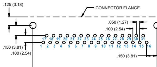
31 SOCKET M83513/19-E
