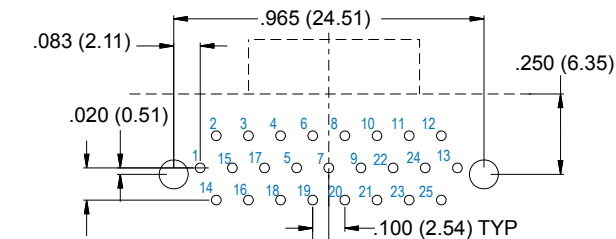
25 PIN
