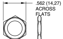
FIGURE C Non-Turn Washer Seal Keyed Washer Hex Nut
