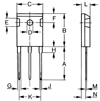
TO-247 AD (IXSH) Outline
