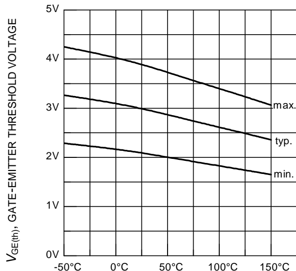
T_j , JUNCTION TEMPERATURE Figure 12. Gate-emitter threshold voltage as a function of junction temperature ( I_C = 0.09\text{mA} )
