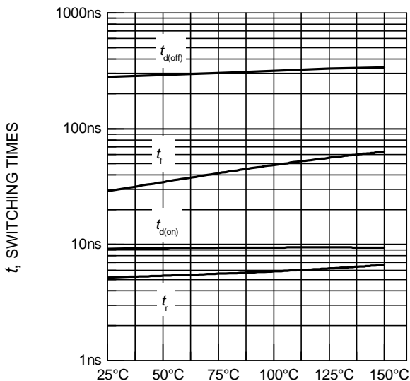
T_j , JUNCTION TEMPERATURE Figure 11. Typical switching times as a function of junction temperature (inductive load, V_{CE} = 800\text{V} , V_{GE} = +15\text{V}/0\text{V} , I_C = 3\text{A} , R_G = 82\Omega , dynamic test circuit in Fig.E)
