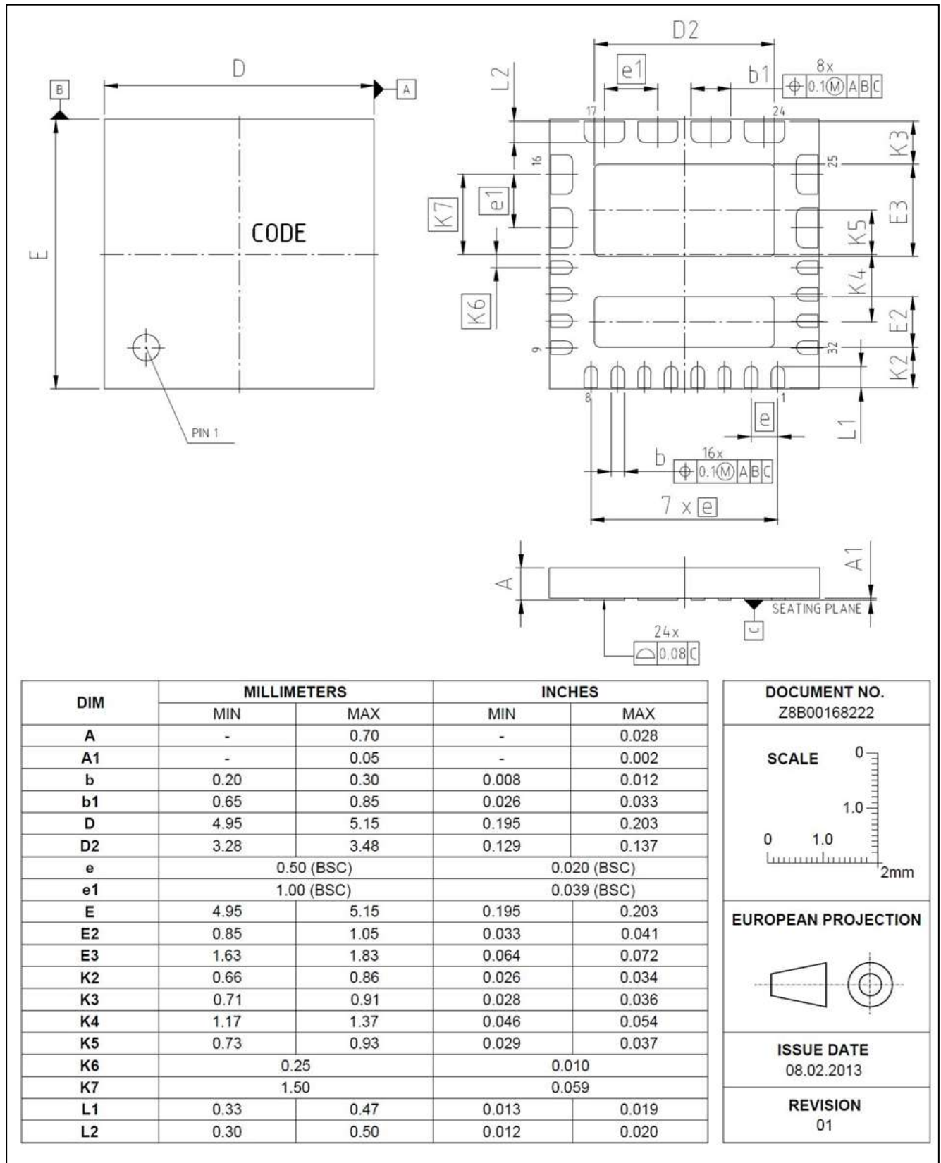
Figure 16 Mechanical dimensions
