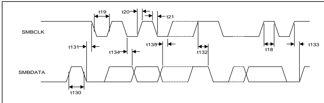
Figure 8-21. SMBus Timeout
