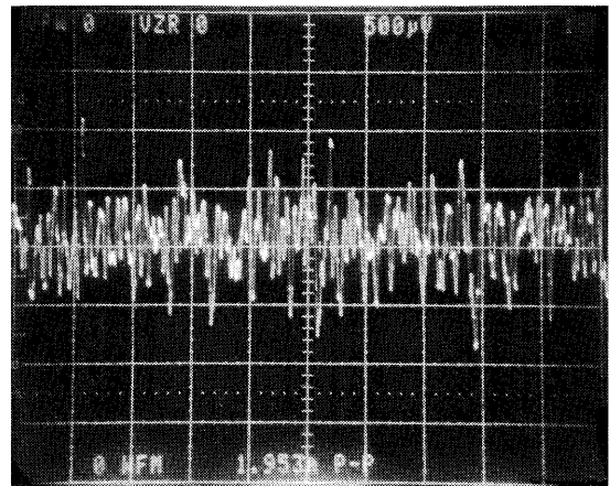
A_{\text{CL}} = 25,000\text{V/V} ; E_{\text{N}} = 0.08\mu\text{V}_{\text{P-P RTI}} Horizontal Scale = 1s/DIV; Vertical Scale = 0.02 \mu\text{V} /DIV
