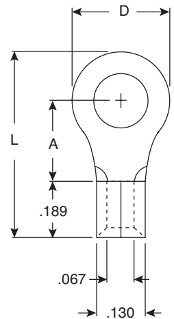
Dimensions: In.
