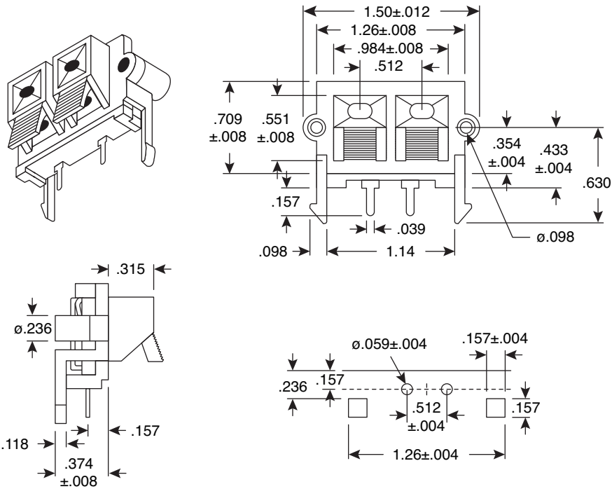
Dimensions: In.
