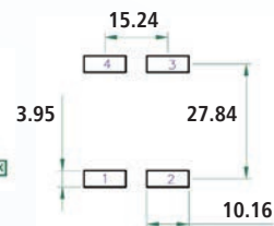
LAND PATTERNS FOR REFLOW SOLDERING
