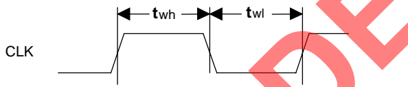
Clock Width
