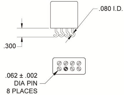
TERMINAL TYPE 2 FINISH: TIN/LEAD PLATE
