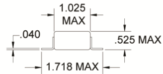
MOUNTING STYLE J
