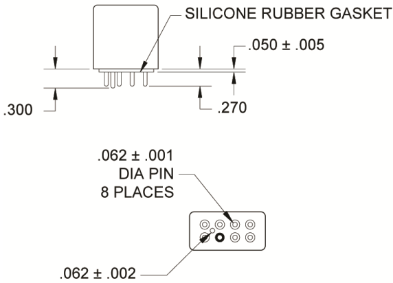
TERMINAL TYPE 4 FINISH: CASE - TIN/LEAD PLATE TERMINAL - GOLD PLATE POLARIZING PIN - TIN/LEAD PLATED
