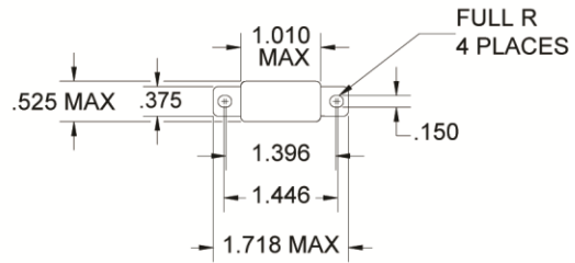
MOUNTING STYLE D
