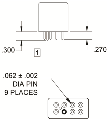
TERMINAL TYPE 1 FINISH: TIN/LEAD PLATE
