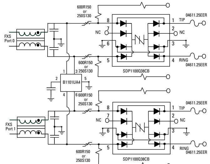
Figure 4.50 FXS Protection
