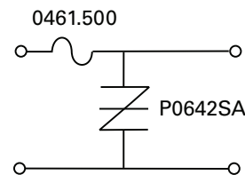
Figure 4.11 T3 Protection – SIDACtor Device
