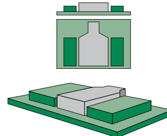
Figure 1.9: NSMD pad
