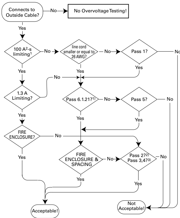
Figure 3.19 Overvoltage Flowchart
