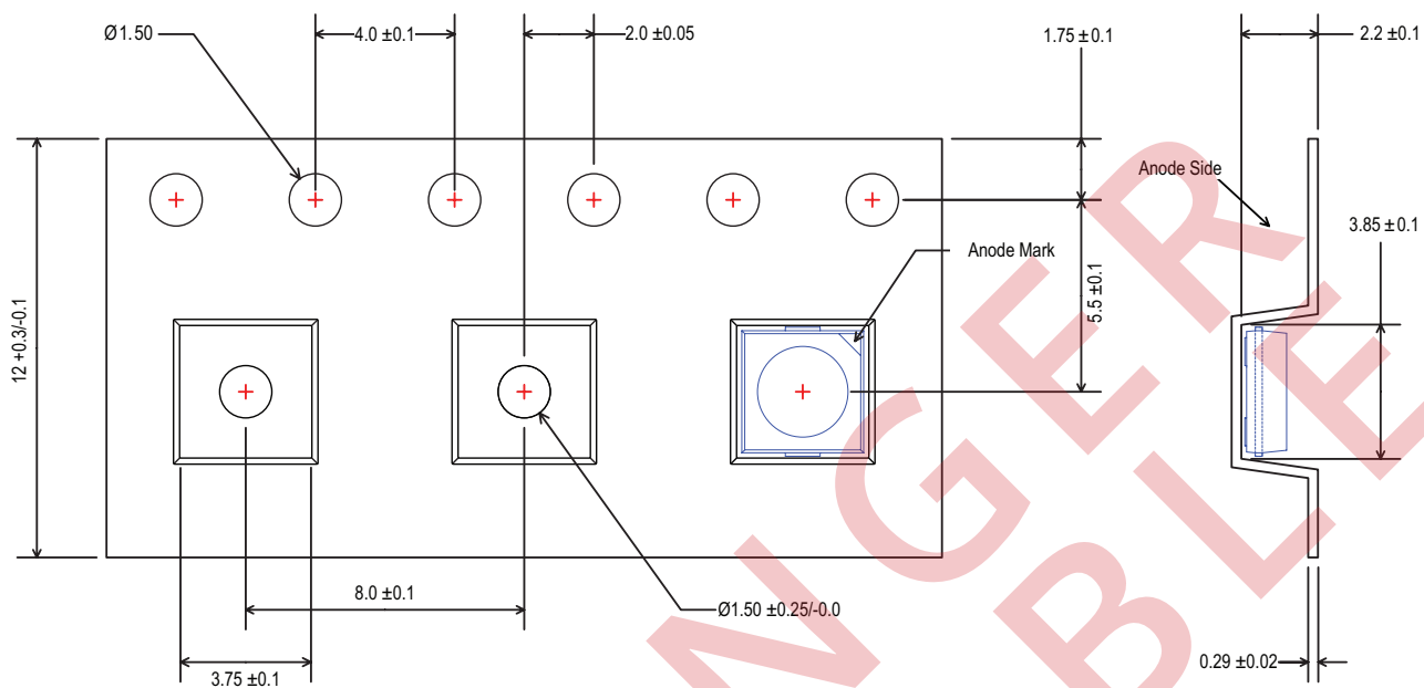
Figure 10. Emitter pocket tape packaging.
