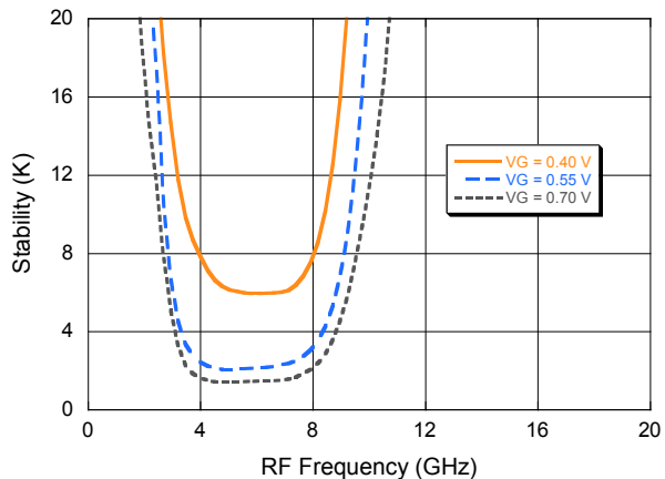
Stability @ -40^\circ\text{C}
