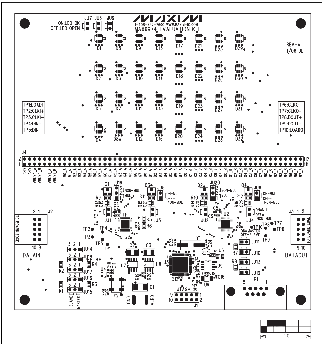
Figure 6. MAX6974 EV Kit Component Placement Guide—Component Side
