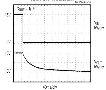
TURN-OFF TRANSIENT
