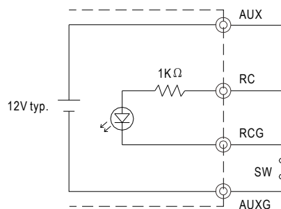
(B) Using internal 12V auxiliary output
