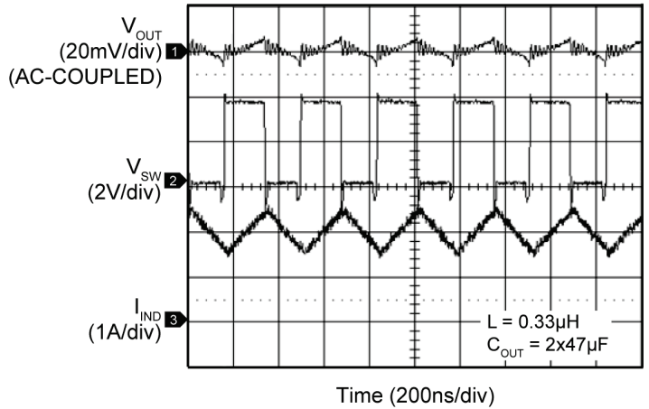
Switching Waveform Continuous Mode (2A)
