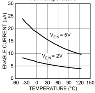
MIC29301-xx/2 Enable Current vs. Temperature
