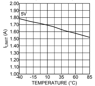
I LIMIT vs. Temperature (MIC20X9 - 0.9A)
