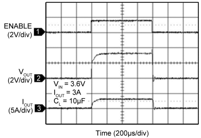
MIC94162/3 Start-Up ( I_{OUT} = 3A )
