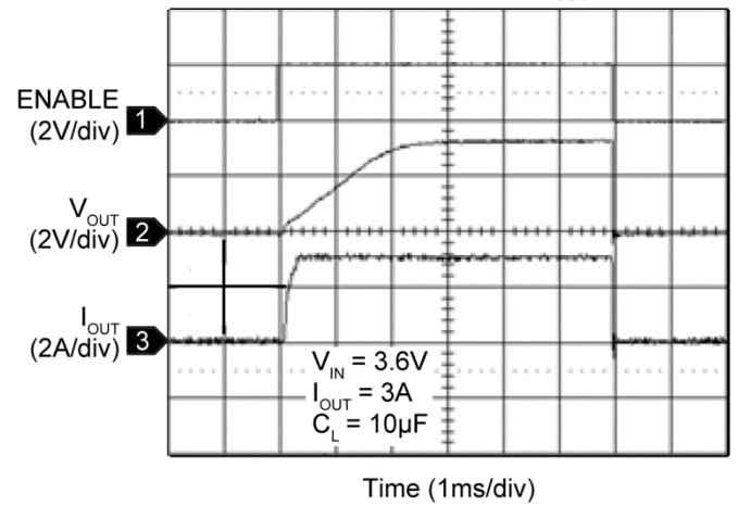
MIC94161/4/5 Start-Up ( I_{OUT} = 3A )
