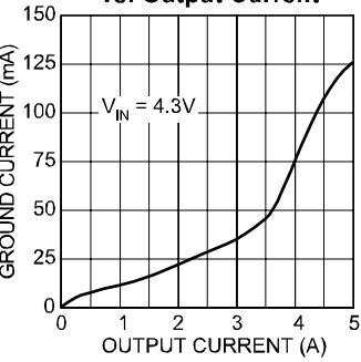
MIC2951x-3.3 Ground Current vs. Output Current
