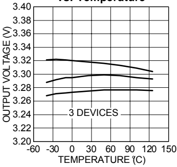
MIC29510-3.3 Output Voltage vs. Temperature
