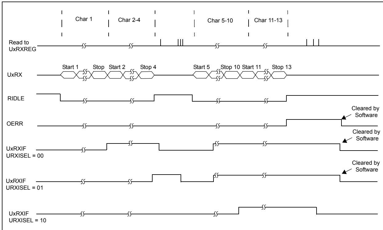
FIGURE 18-2: UART RECEPTION
