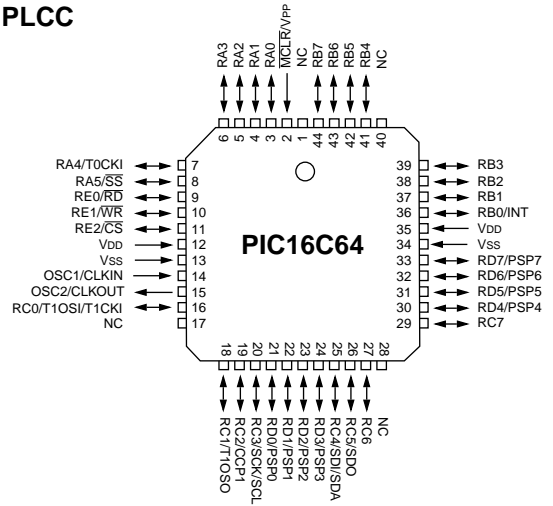
PLCC
