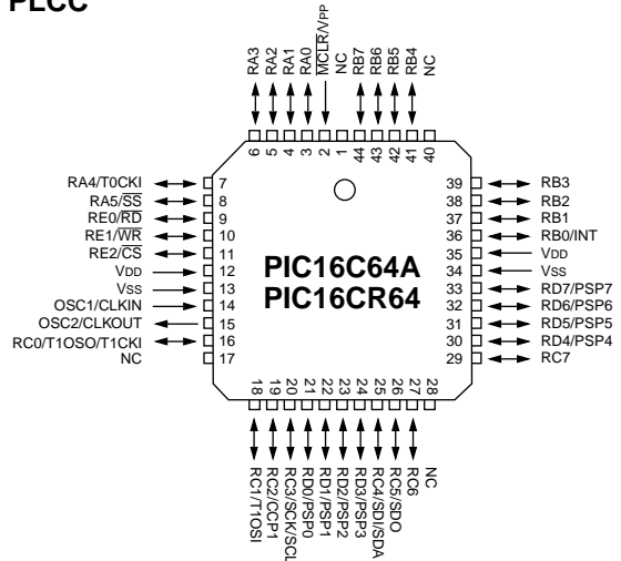
PLCC
