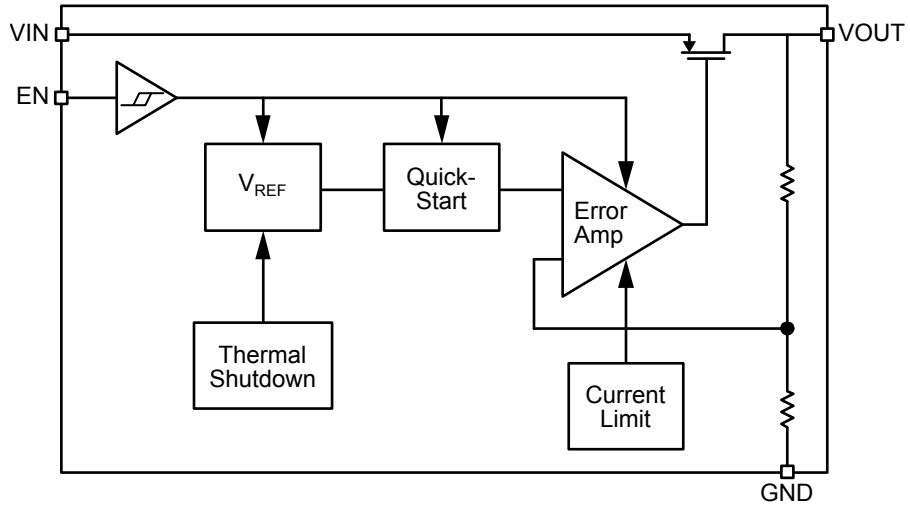
MIC5302 Block Diagram
