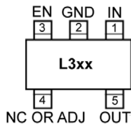
5-Pin SOT-23 (M5)
