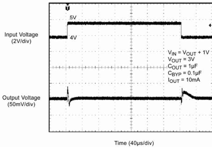
Line Transient
