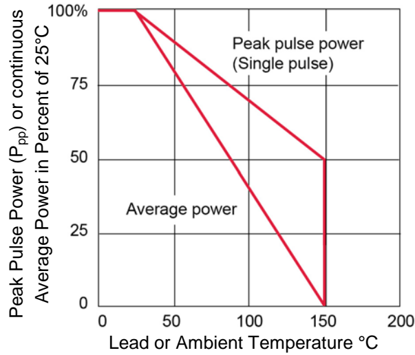
FIGURE 3 Derating Curve
