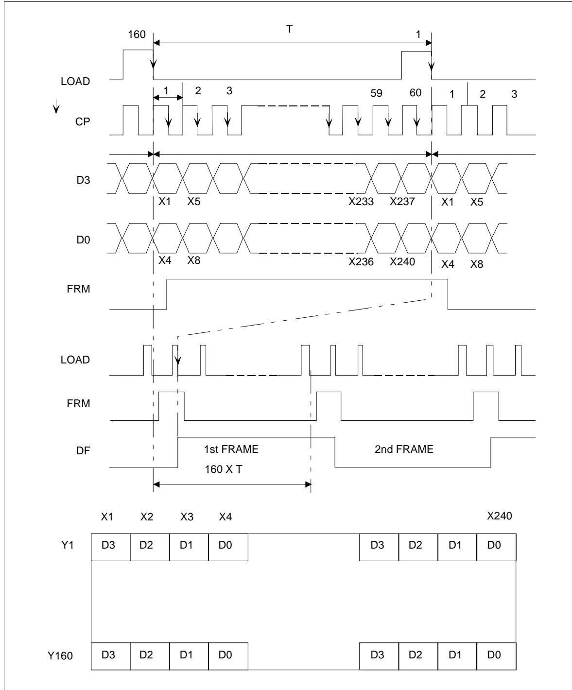
Signal Timing (2)
