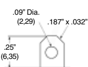
S 1 Solder Eye & Quick Connect (Standard)
