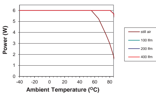
NCM6X1205C
