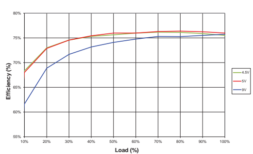
NCM6S0503C
