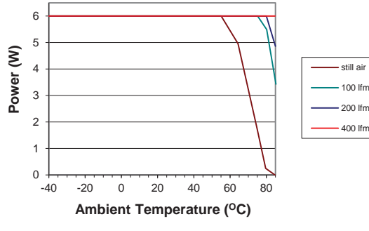
NCM6X1212C
