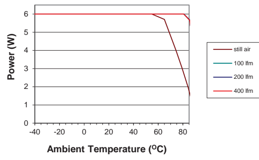
NCM6X0515C
