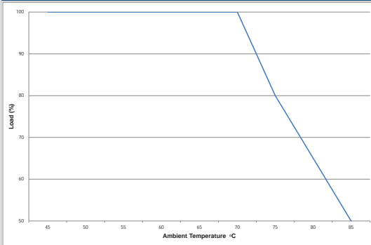
MTU2D1212MC
