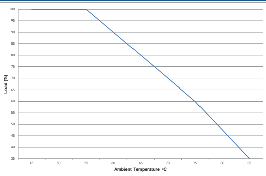
MTU2D0512MC
