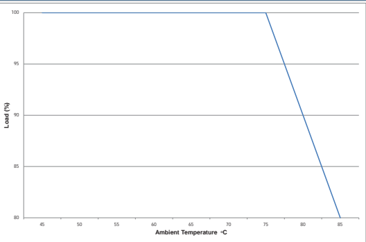
MTU2S2405MC
