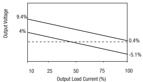
MTU2S0524MC
