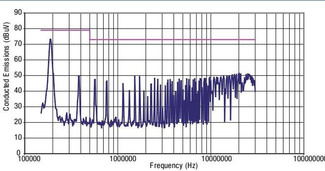
NCS6D4812C
