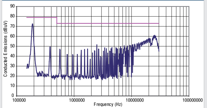
NCS6D4805C
