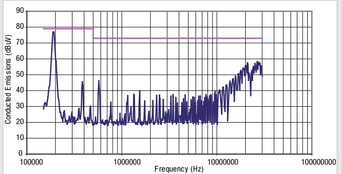
NCS6D1212C
