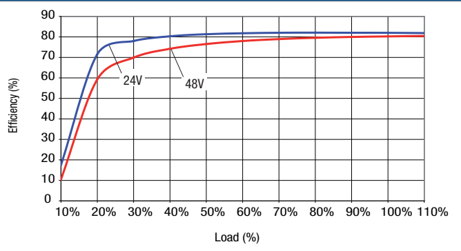
NCS6S4815C
