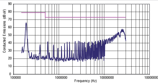
NCS6D1205C
