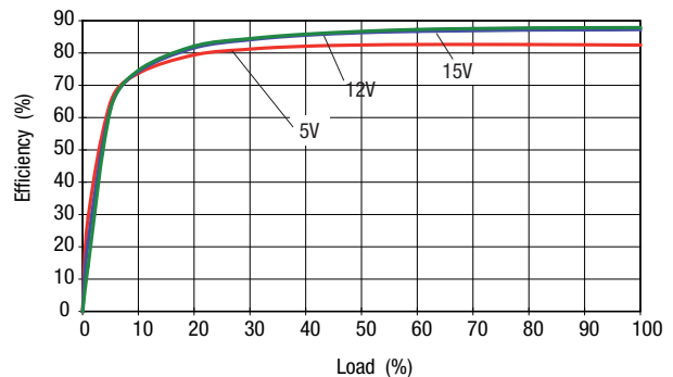
NDS 24V Input, Single Output
